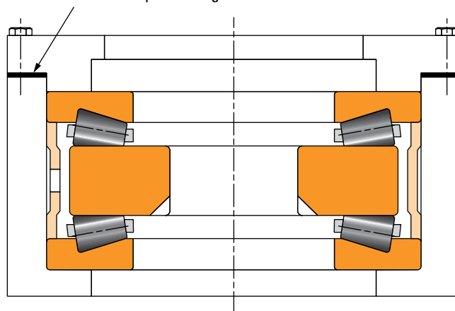
Fig. 45. TTDFLK thrust bearing mounted in housing.
