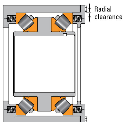
Fig. 36. Back-to-back mounting arrangement of a TSR-EM bearing set.
