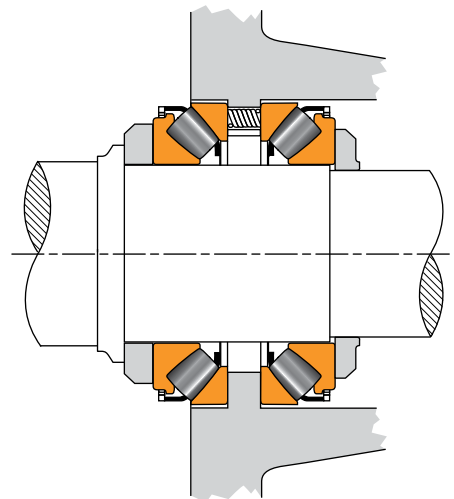
Fig. 35. Face-to-face mounting arrangement of a TSR-EJ bearing set.
